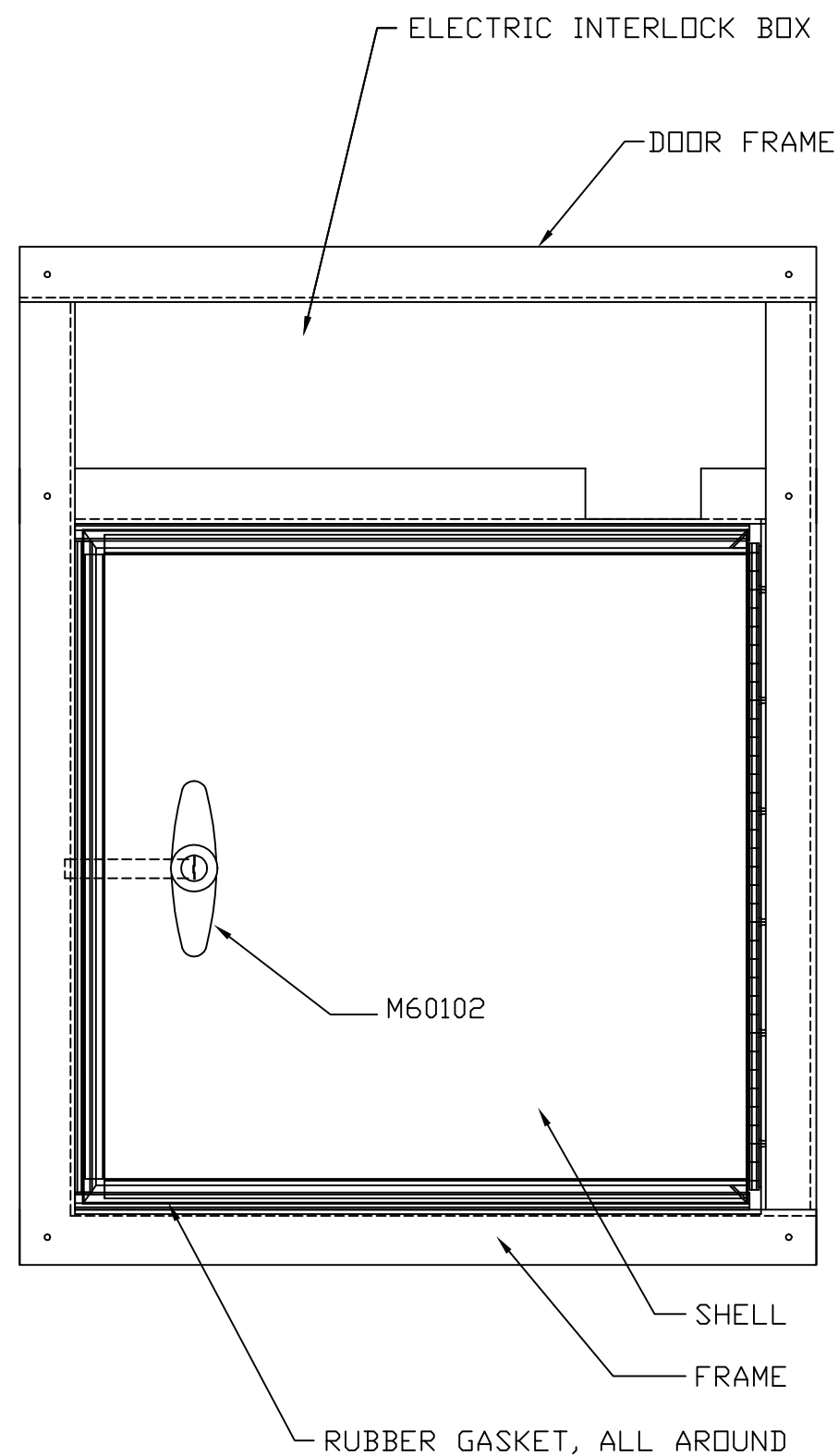
SIDE HINGED HAND OPERATED CHUTE INTAKE DOOR-ELECTRICALLY INTERLOCKED
